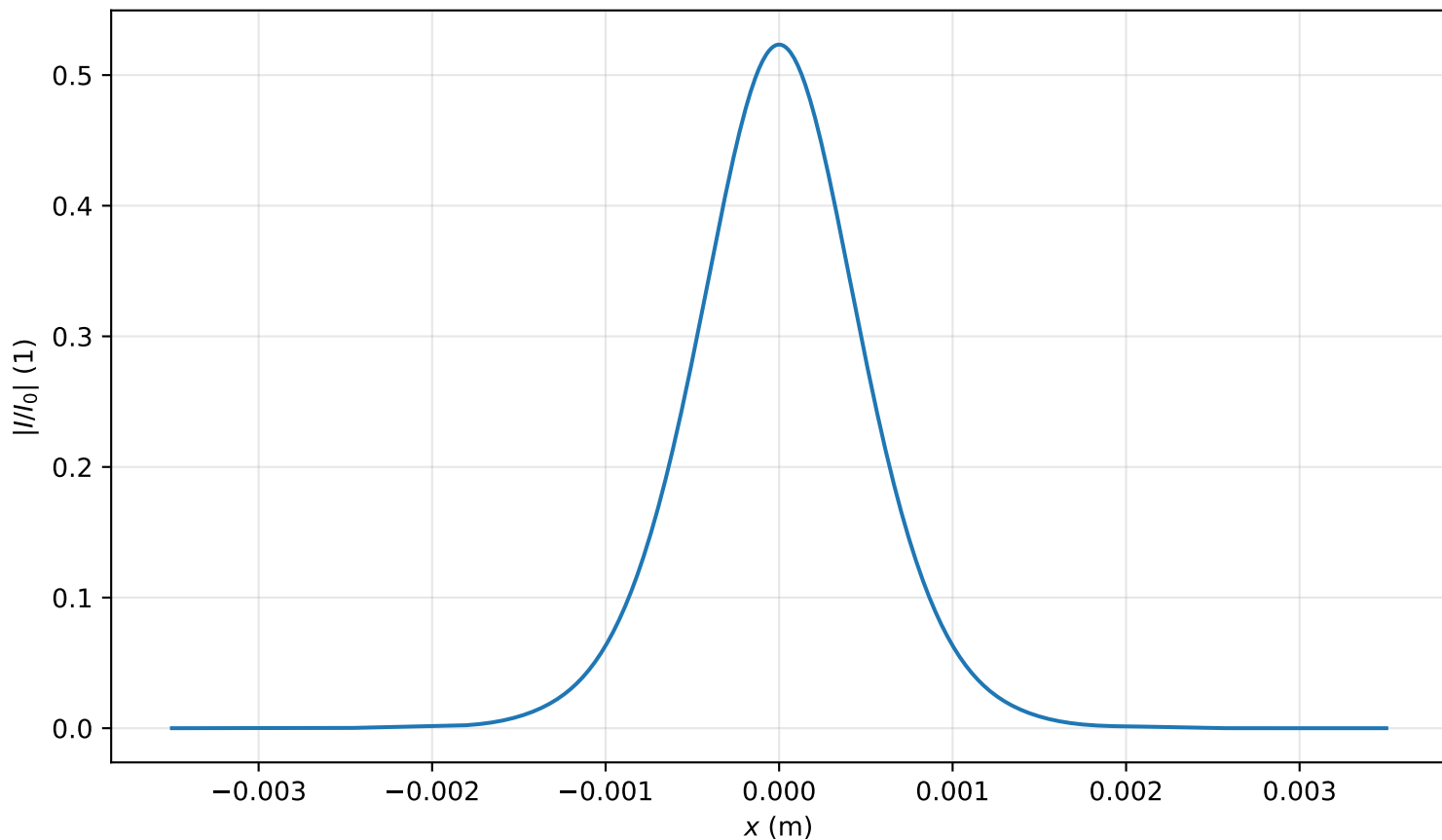
Intensity profile I(x, y = 0, z = 3.742m)/I_0 , P_{in}=0.6P_{cr} , artificial time
